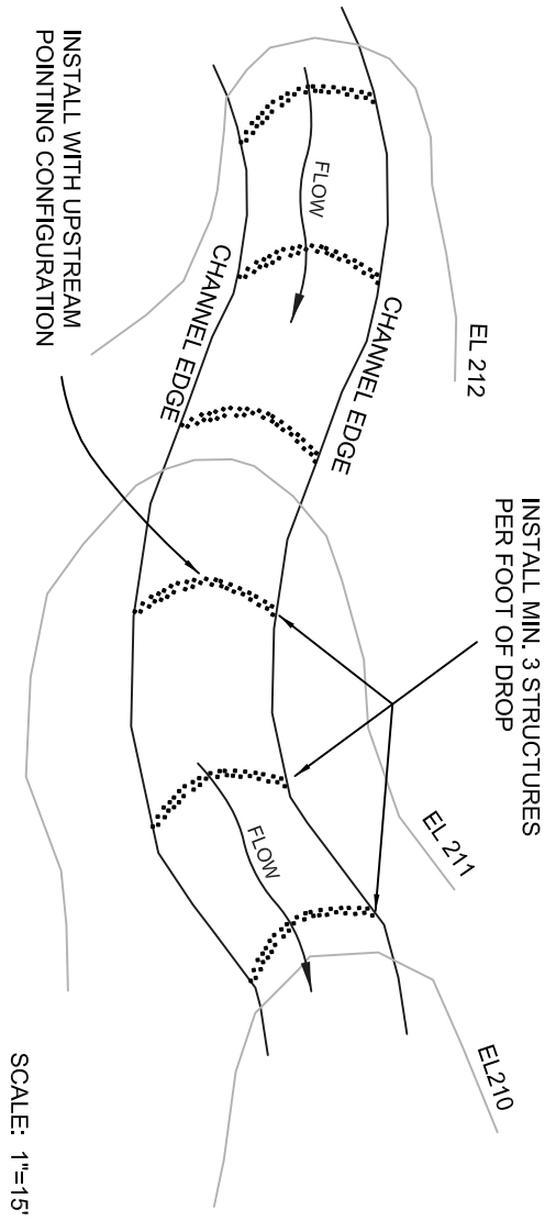
FIGURE 4 -- STRUCTURE SPACING AND SHAPE
